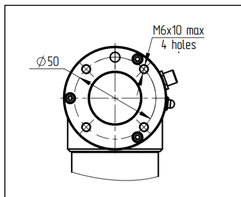
Figure 2-3: Basic mechanical interface on the arm wrist
