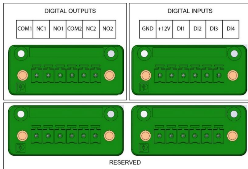
Figure 1-11: Pin assignment for digital I/O connectors
